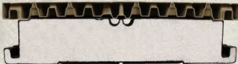
Dock Section Top and Bottom (Interior View); Foam-Filled Bottom Float
